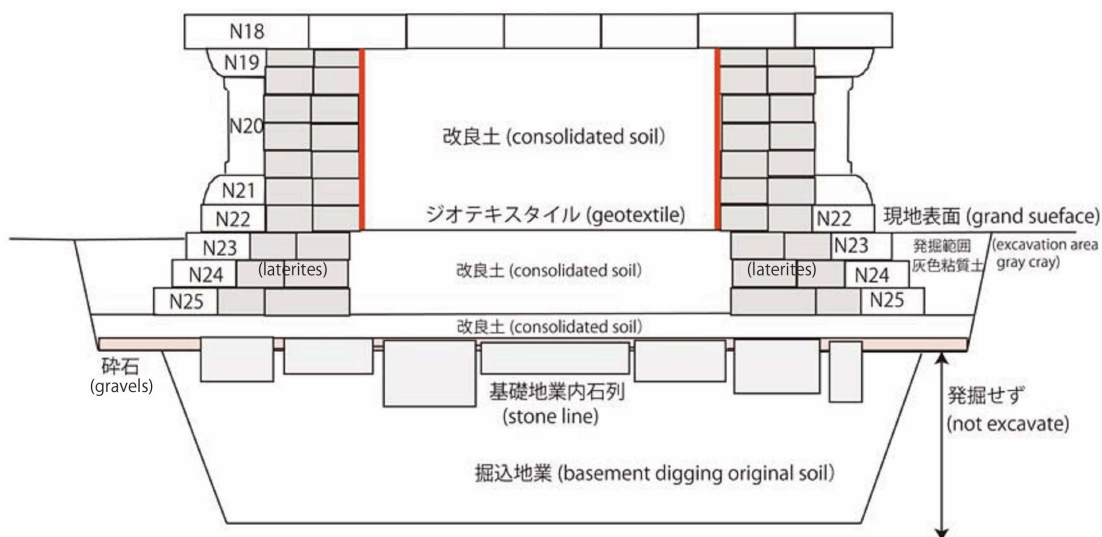
南祠堂の下成基壇の再構築モデル図 Reassembling plan of the lower foundation of the Southern Sanctuary
