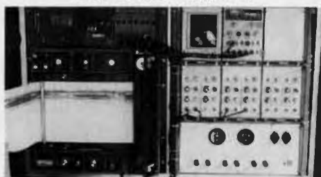
*31 OYO Geo-Radar II
