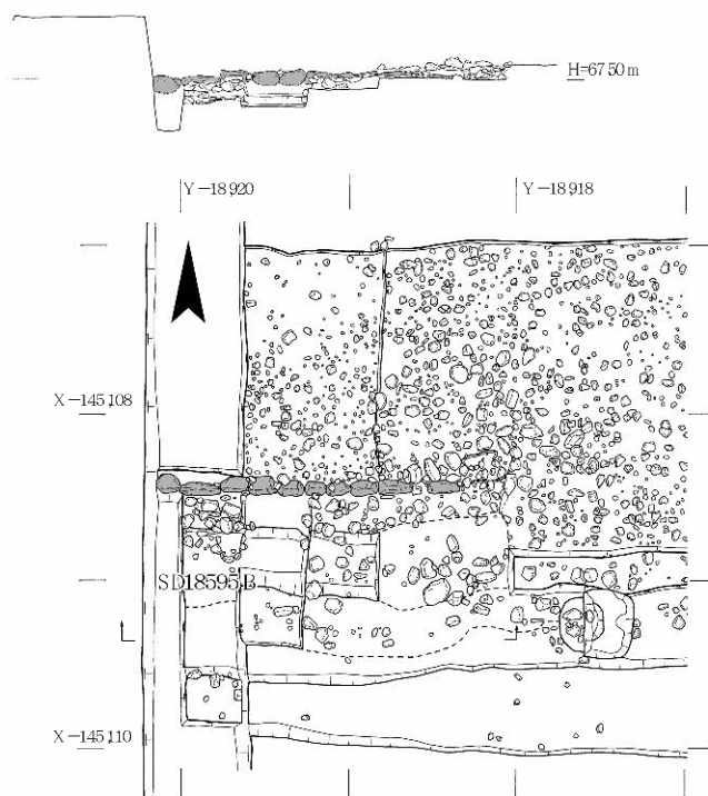
図52 見切石列SX18600 1:50
